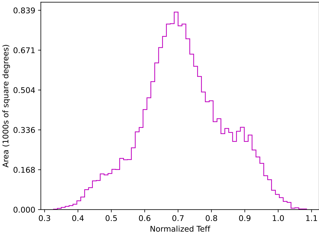
too_ignore_5_1v3.4_10yrs WFD z band: Normalized Teff
