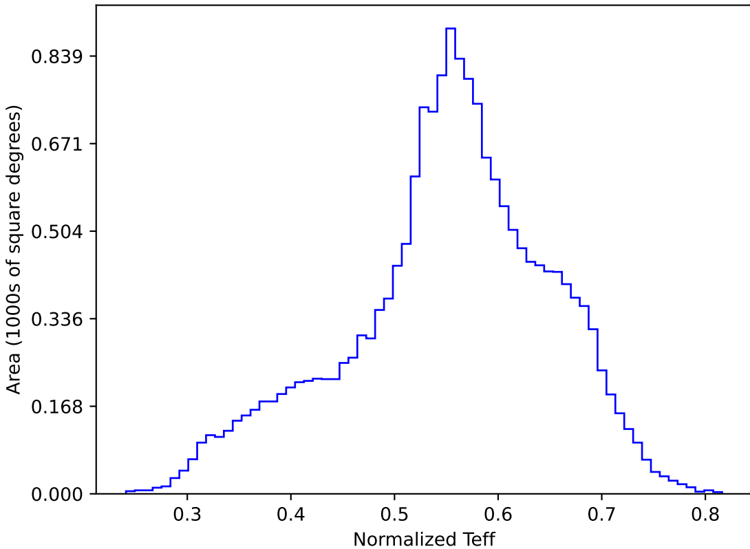
too_ignore_5_1v3.4_10yrs WFD y band: Normalized Teff
