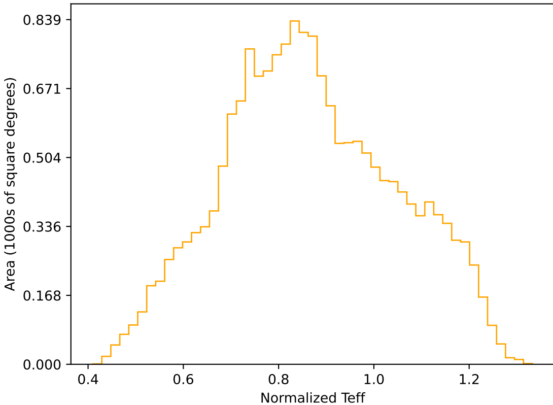
too_ignore_5_1v3.4_10yrs WFD r band: Normalized Teff
