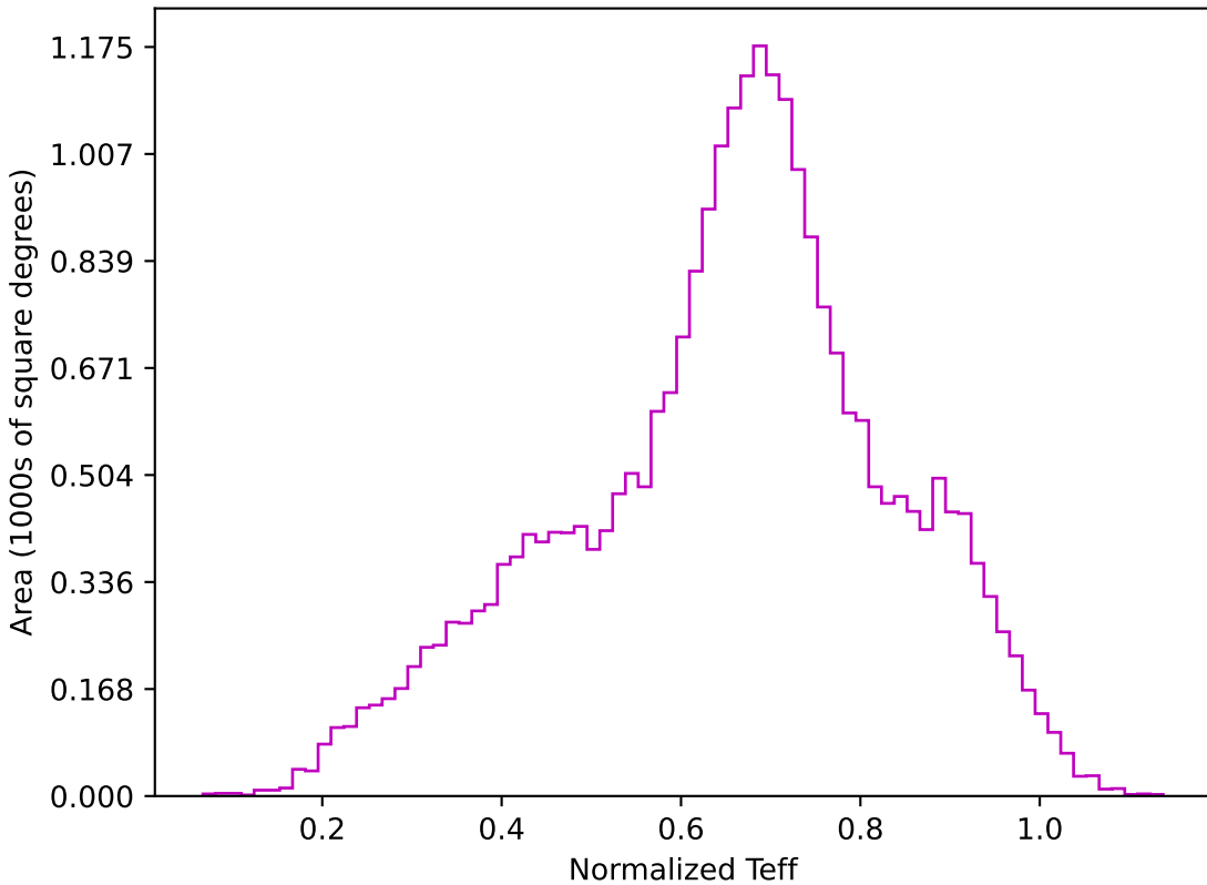
too_ignore_5_1v3.4_10yrs All sky z band: Normalized Teff
