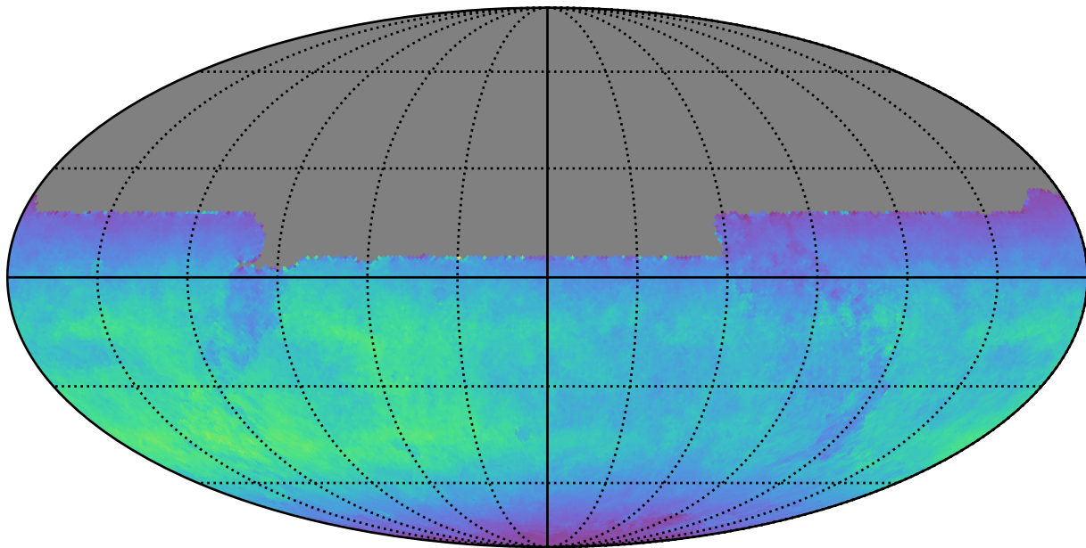
too_ignore_5_1v3.4_10yrs All sky y band: Normalized Teff
