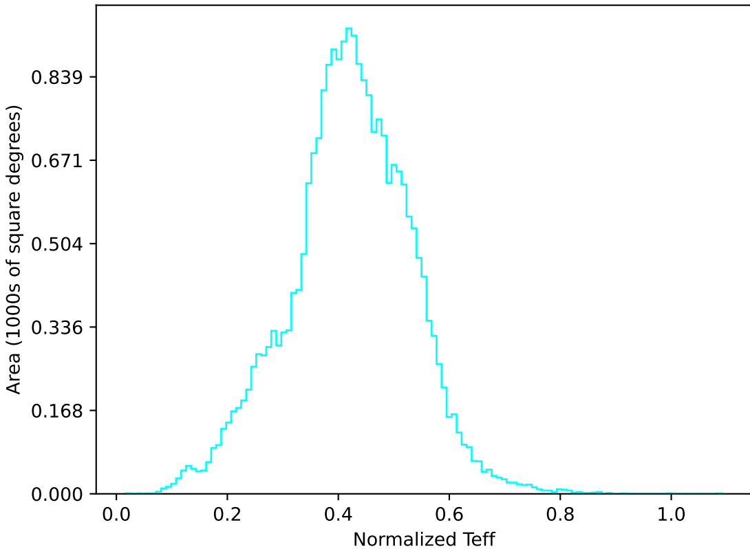
too_ignore_5_1v3.4_10yrs All sky u band: Normalized Teff
