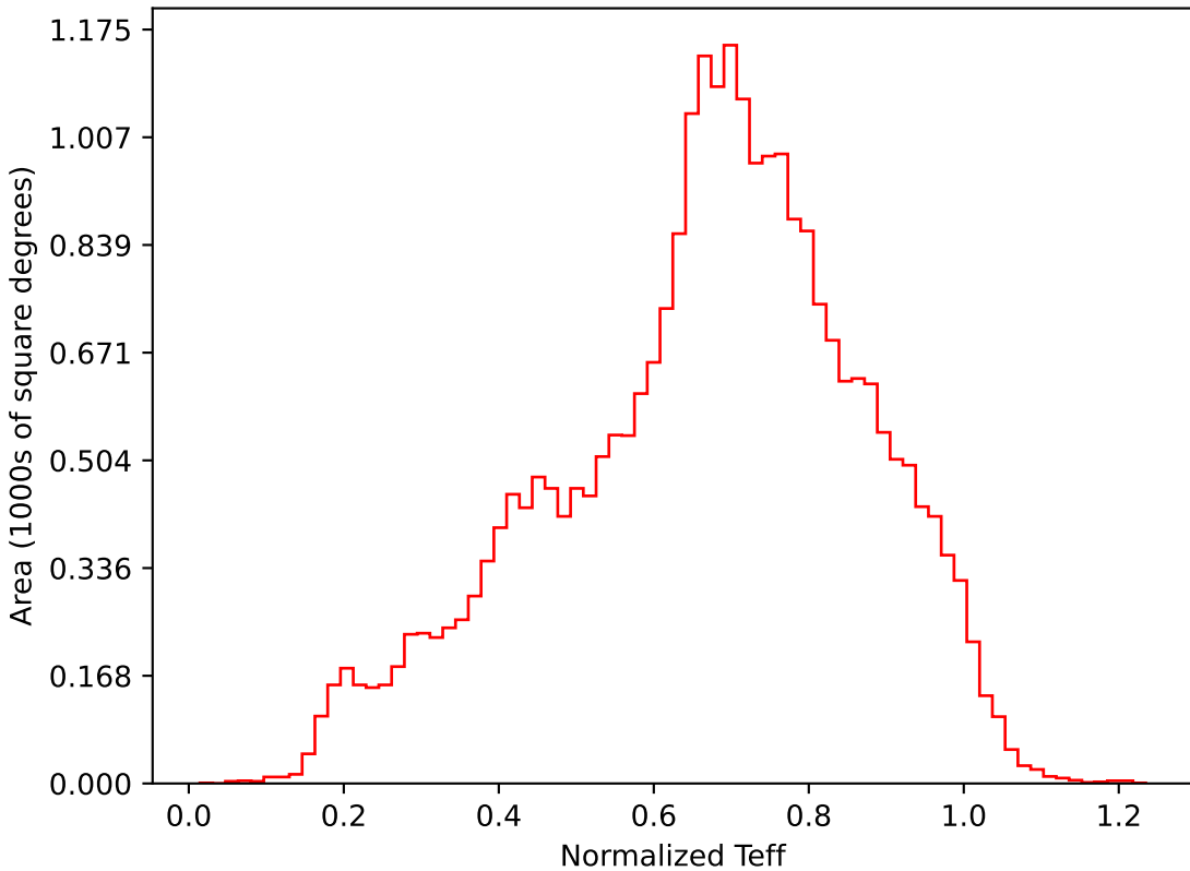
too_ignore_5_1v3.4_10yrs All sky i band: Normalized Teff
