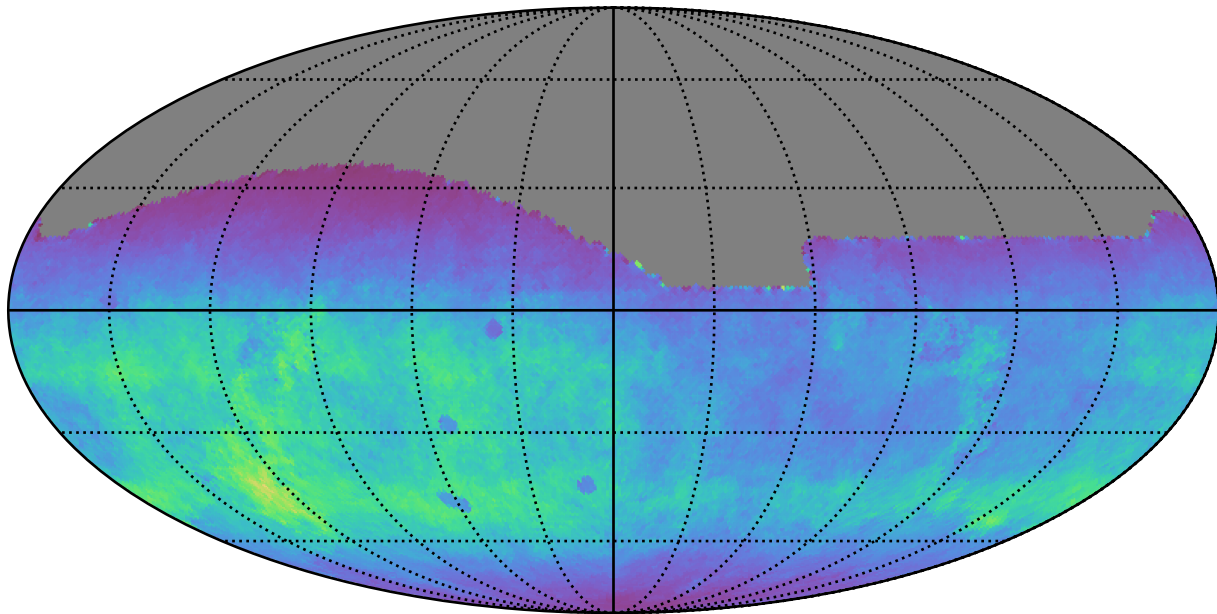
too_ignore_5_1v3.4_10yrs All sky g band: Normalized Teff
