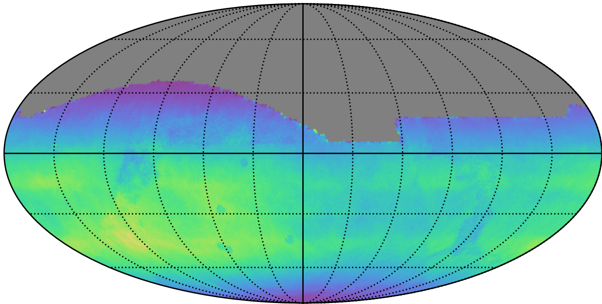
too_ignore_5_1v3.4_10yrs All sky all bands: Normalized Teff
