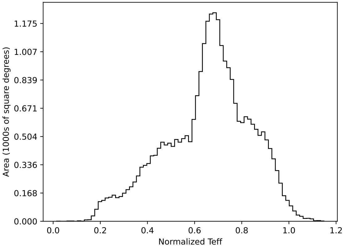
too_ignore_5_1v3.4_10yrs All sky all bands: Normalized Teff
