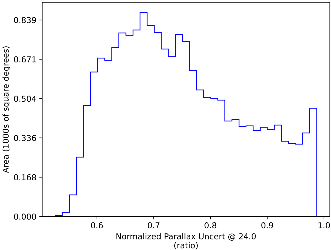
too_ignore_5_1v3.4_10yrs WFD: Normalized Parallax Uncert @ 24.0
