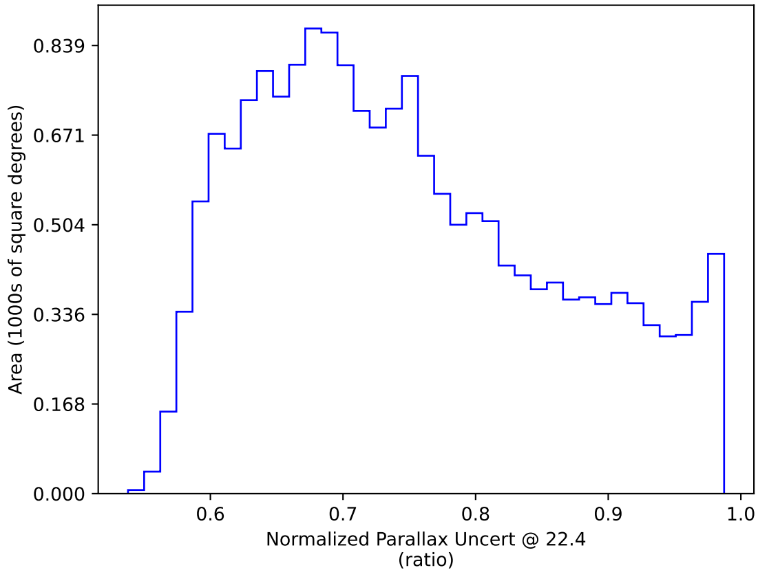
too_ignore_5_1v3.4_10yrs WFD: Normalized Parallax Uncert @ 22.4
