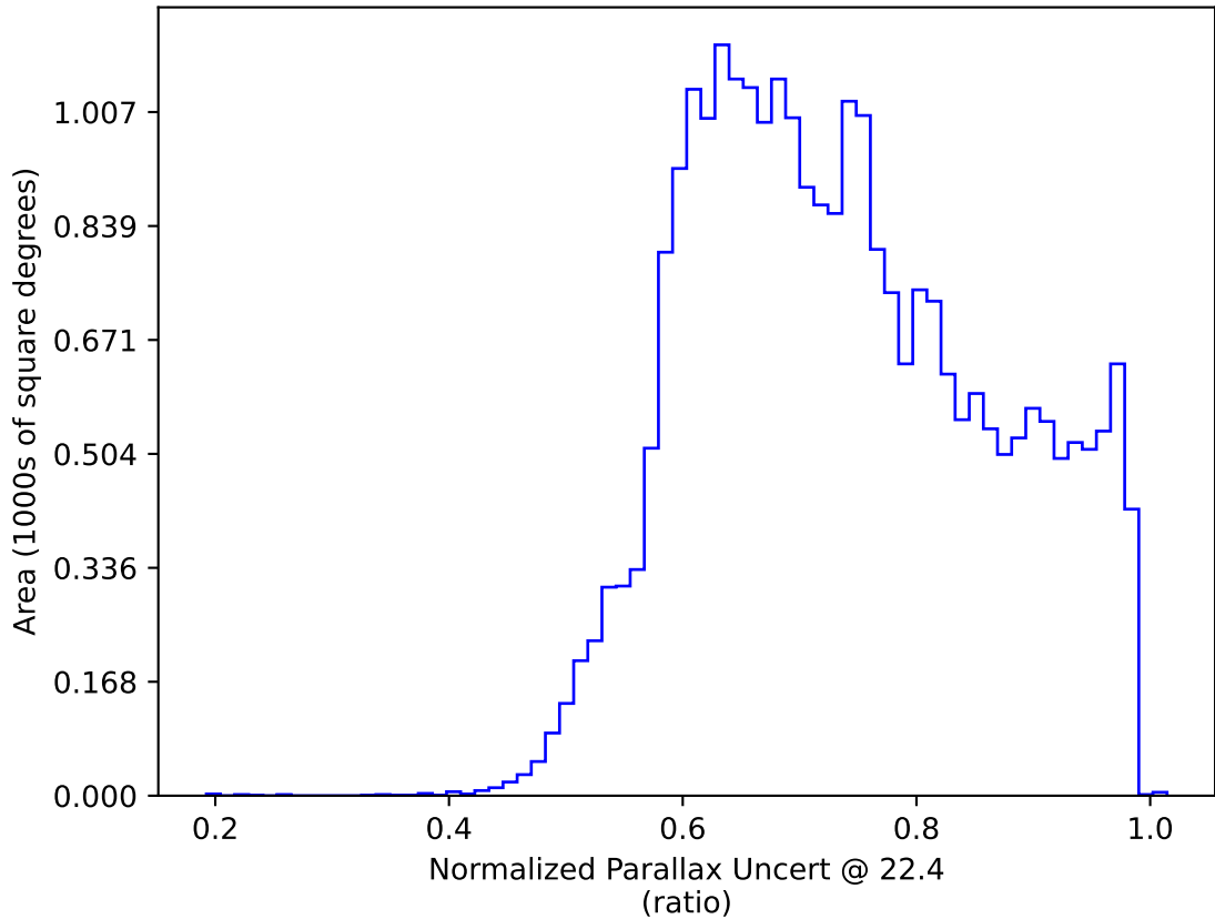
too_ignore_5_1v3.4_10yrs All sky: Normalized Parallax Uncert @ 22.4
