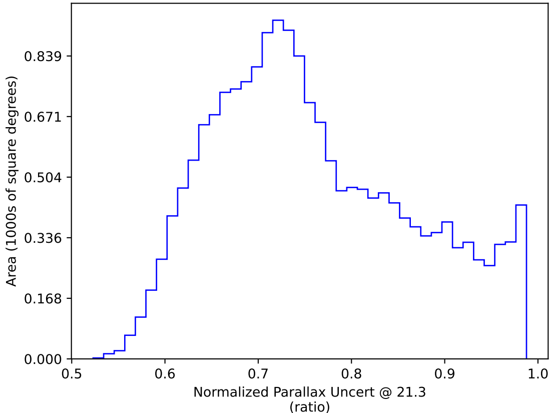
too_ignore_5_1v3.4_10yrs WFD y band only: Normalized Parallax Uncert @ 21.3
