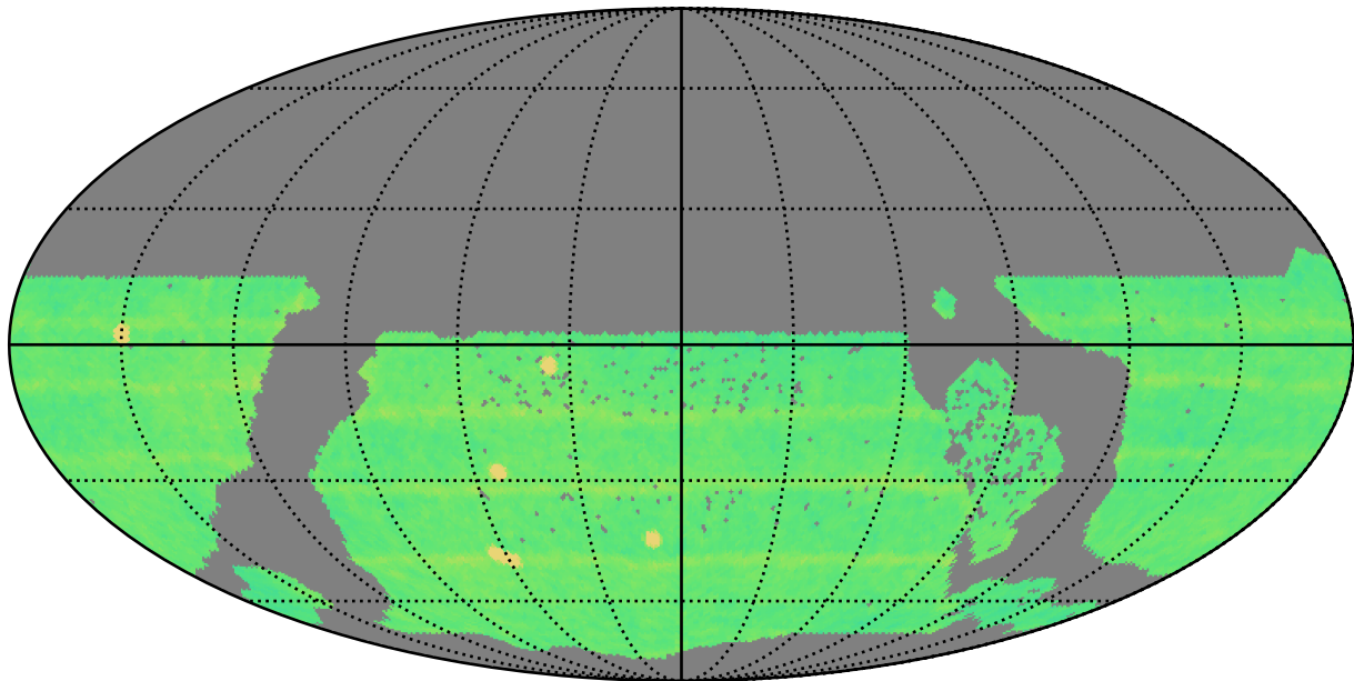
too_ignore_5_1v3.4_10yrs WFD all bands: N Unique Nights
