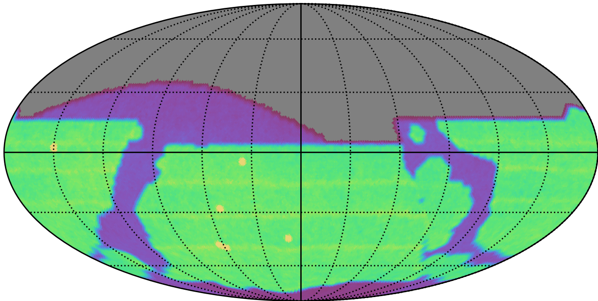
too_ignore_5_1v3.4_10yrs All sky all bands: N Unique Nights
