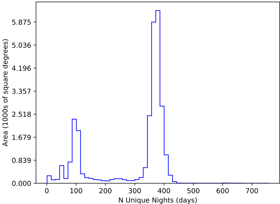
too_ignore_5_1v3.4_10yrs All sky all bands: N Unique Nights
