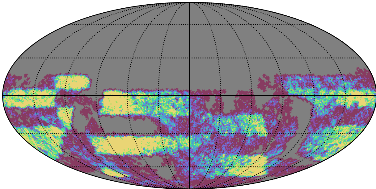
too_ignore_5_1v3.4_10yrs Yr 3-4 u band: NVisits
