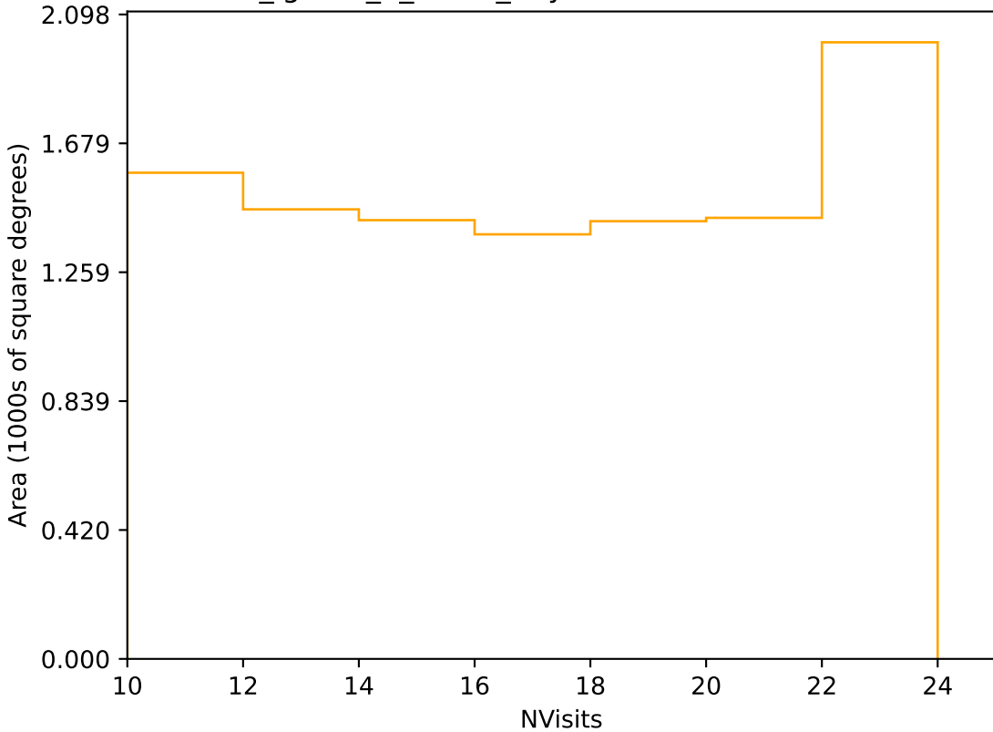
too_ignore_5_1v3.4_10yrs Yr 3-4 r band: NVisits
