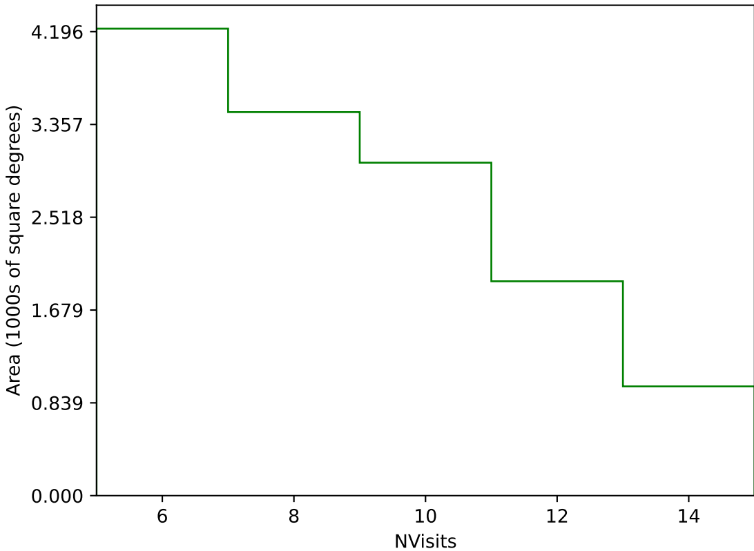
too_ignore_5_1v3.4_10yrs Yr 3-4 g band: NVisits
