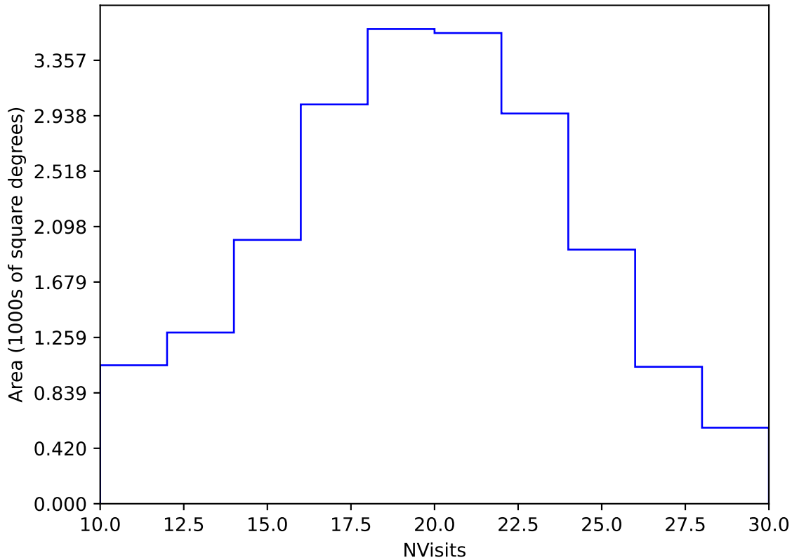
too_ignore_5_1v3.4_10yrs Yr 1 y band: NVisits
