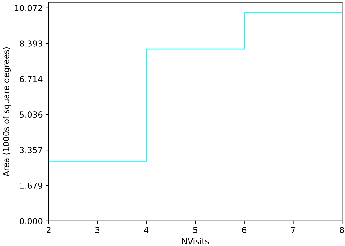
too_ignore_5_1v3.4_10yrs Yr 1 u band: NVisits
