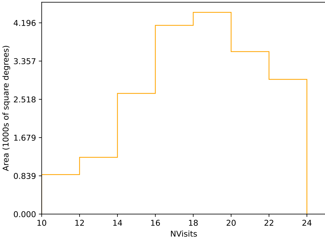
too_ignore_5_1v3.4_10yrs Yr 1 r band: NVisits
