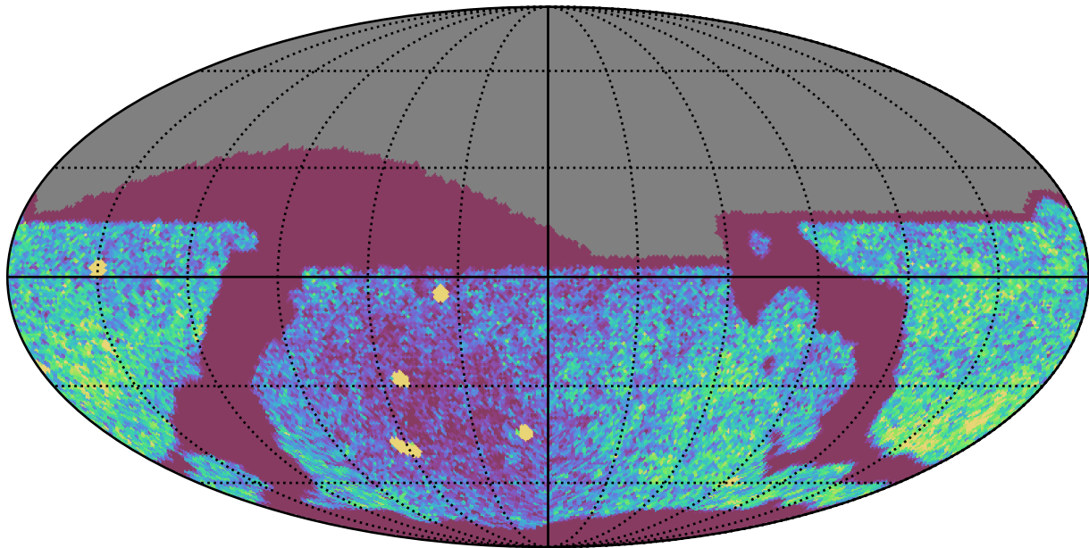
too_ignore_5_1v3.4_10yrs Yr 1 all bands: NVisits
