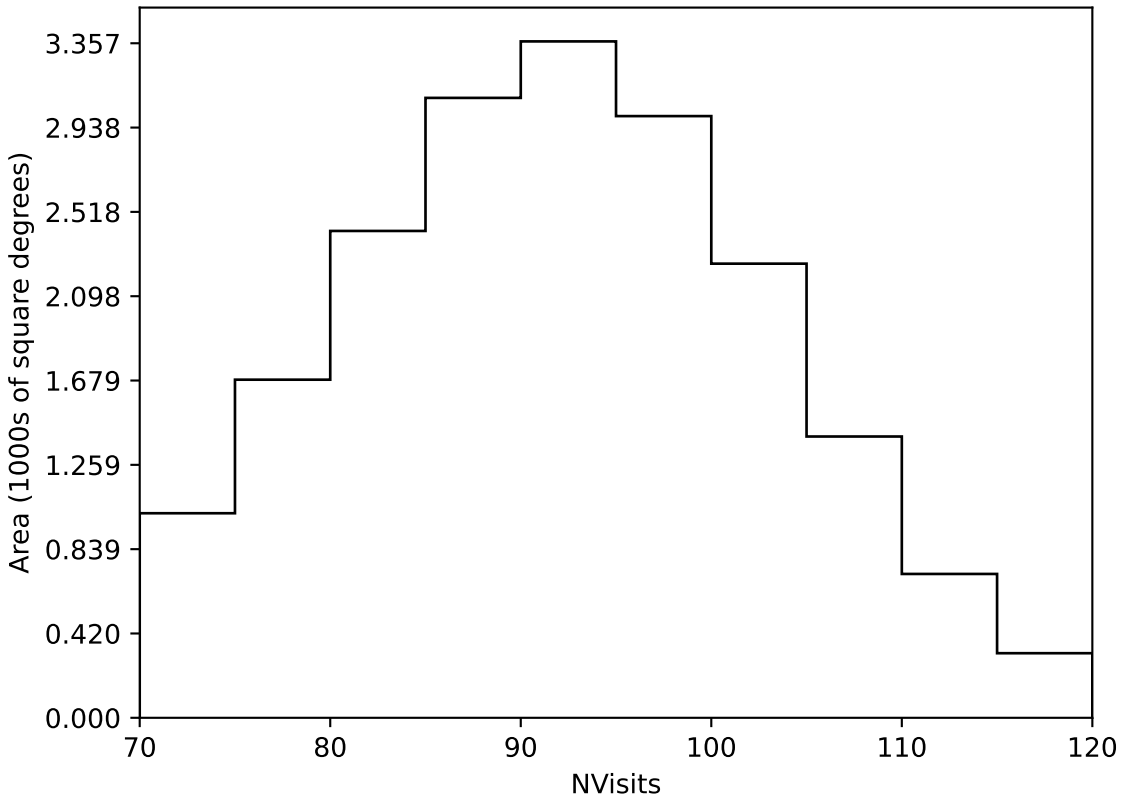
too_ignore_5_1v3.4_10yrs Yr 1 all bands: NVisits
