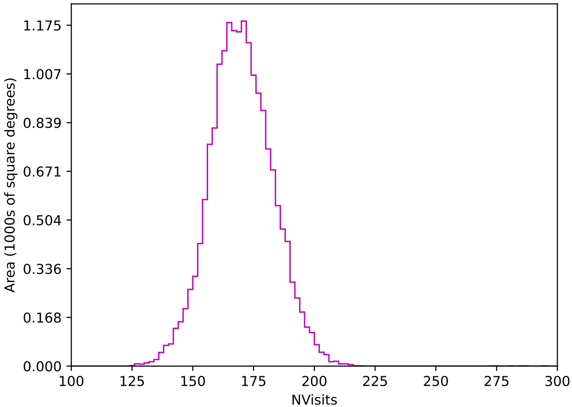
too_ignore_5_1v3.4_10yrs WFD z band: NVisits
