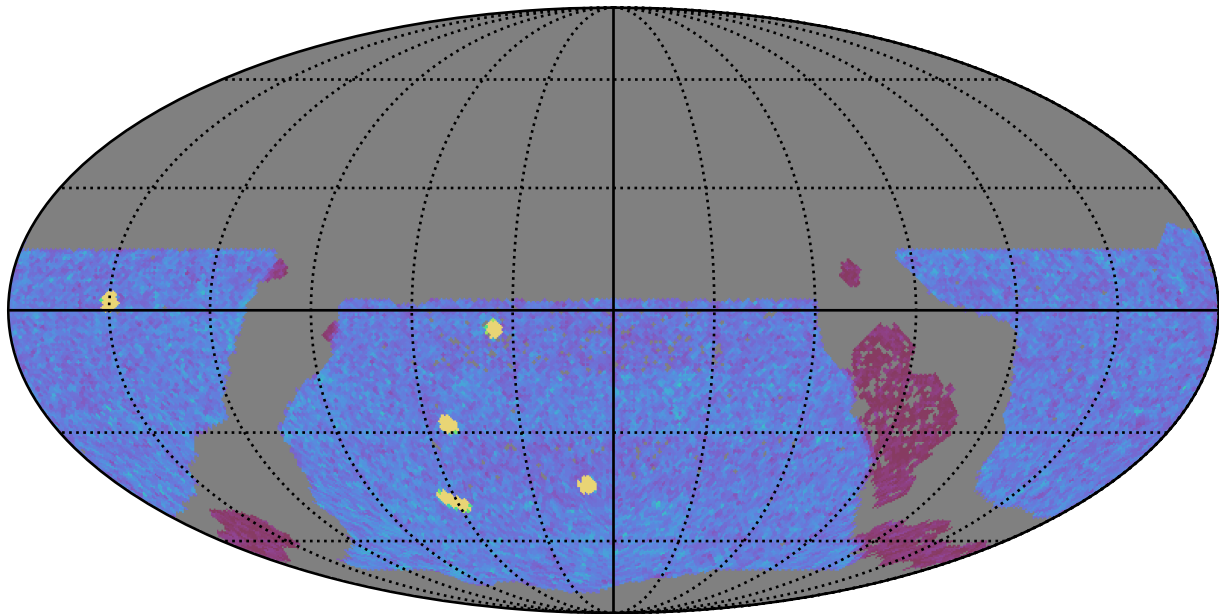
too_ignore_5_1v3.4_10yrs WFD y band: NVisits
