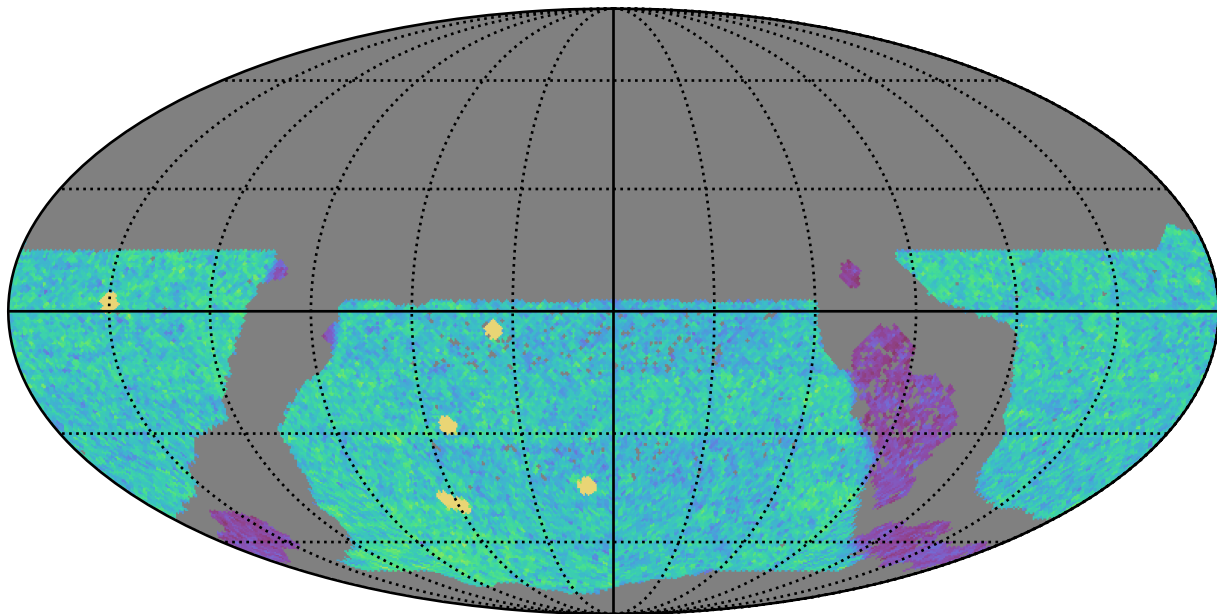
too_ignore_5_1v3.4_10yrs WFD u band: NVisits
