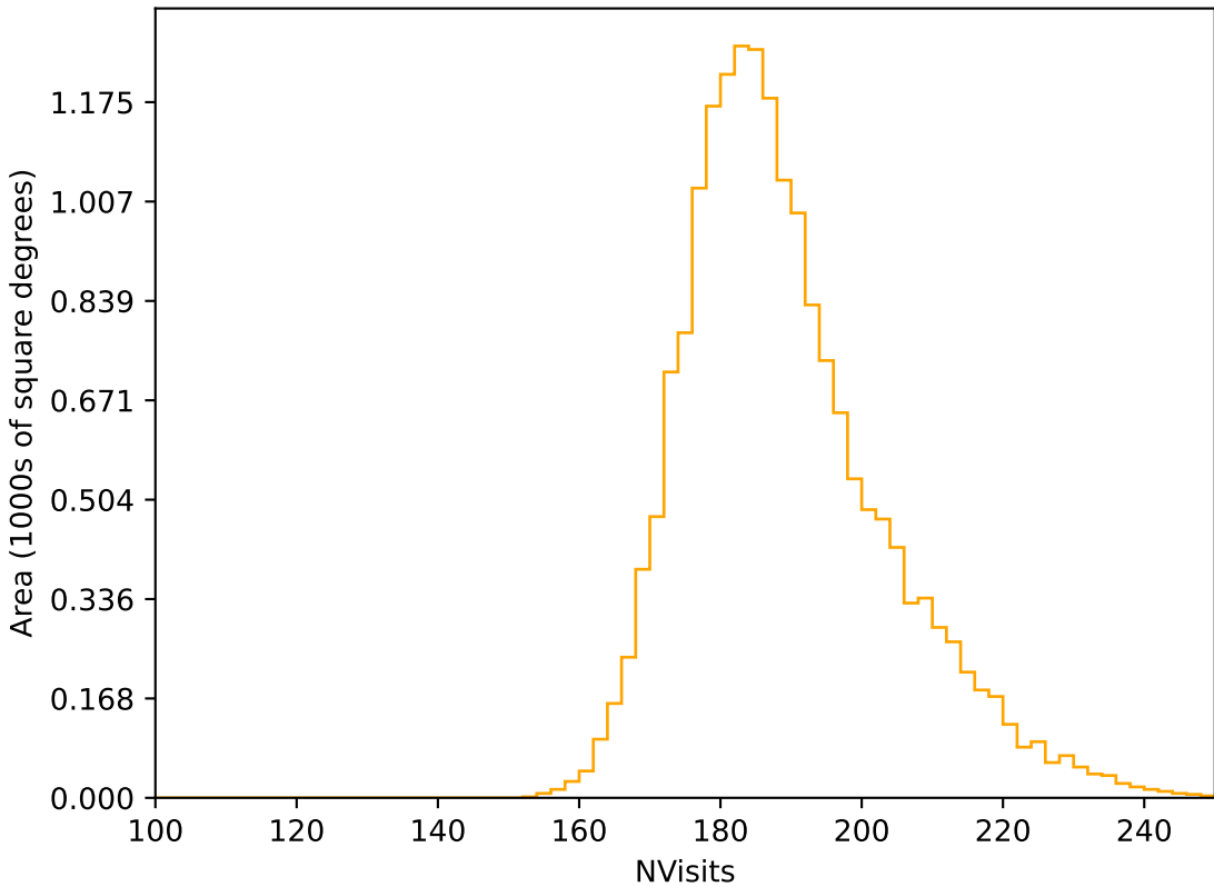
too_ignore_5_1v3.4_10yrs WFD r band: NVisits
