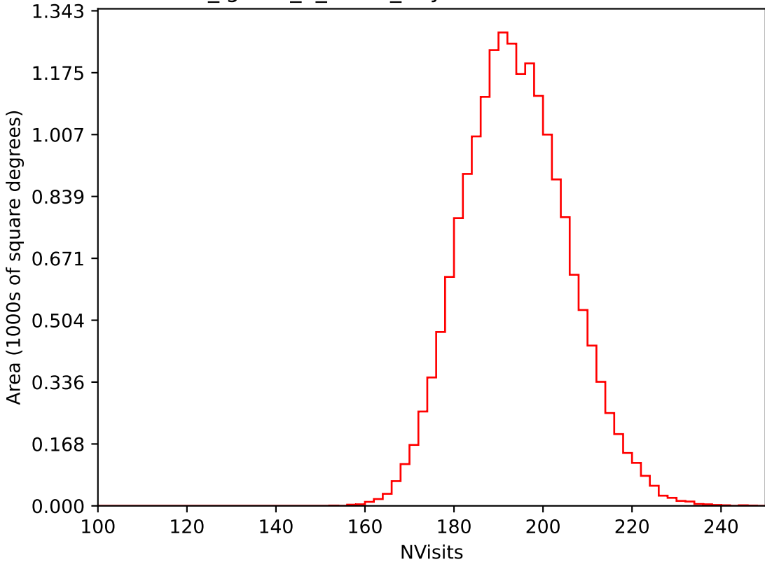
too_ignore_5_1v3.4_10yrs WFD i band: NVisits
