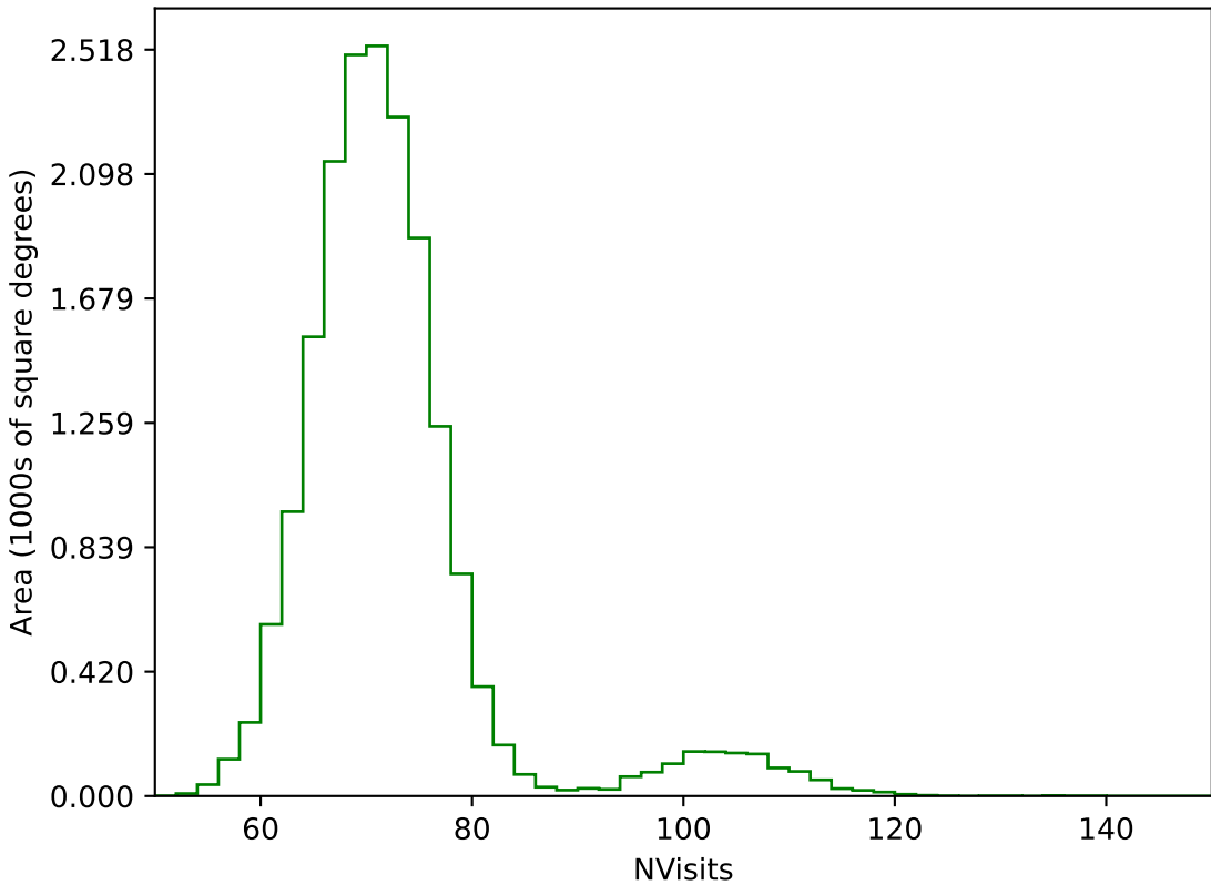
too_ignore_5_1v3.4_10yrs WFD g band: NVisits
