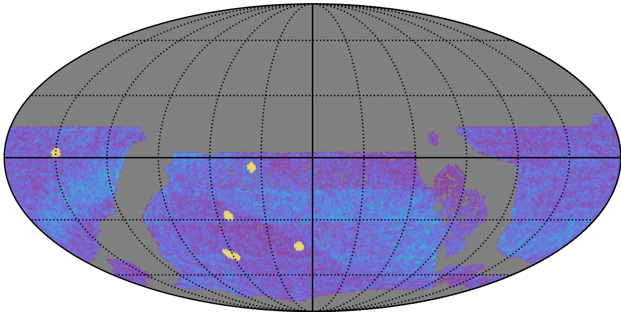
too_ignore_5_1v3.4_10yrs WFD all bands: NVisits
