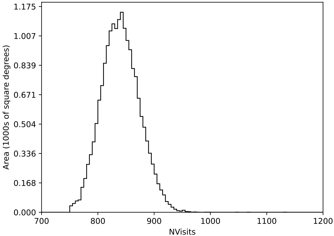
too_ignore_5_1v3.4_10yrs WFD all bands: NVisits
