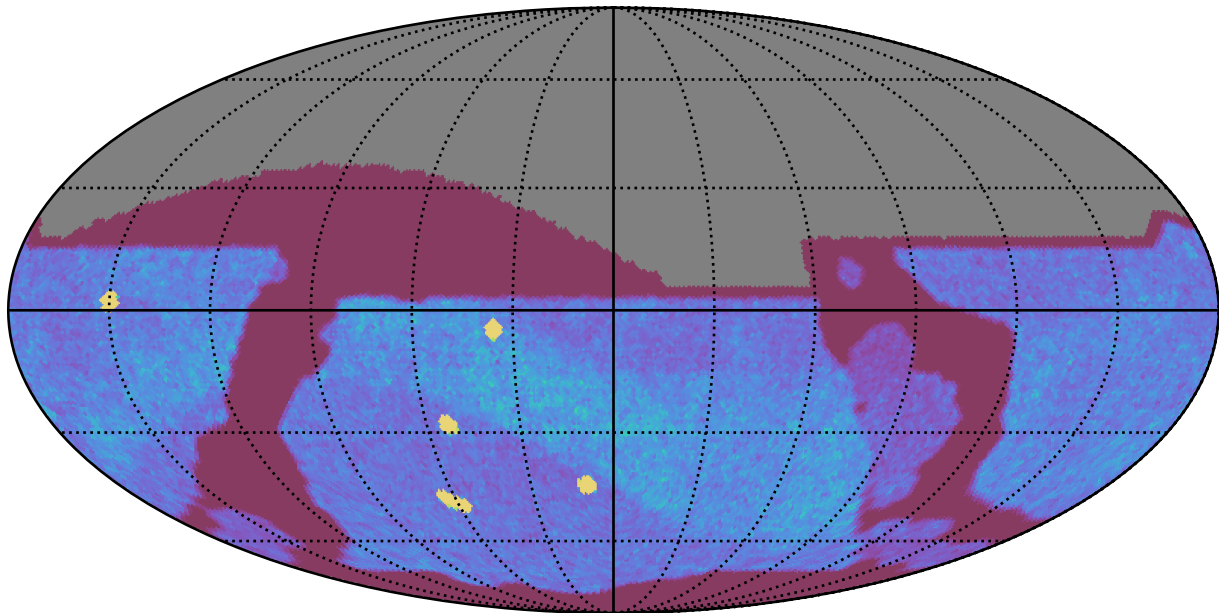
too_ignore_5_1v3.4_10yrs All sky z band: NVisits
