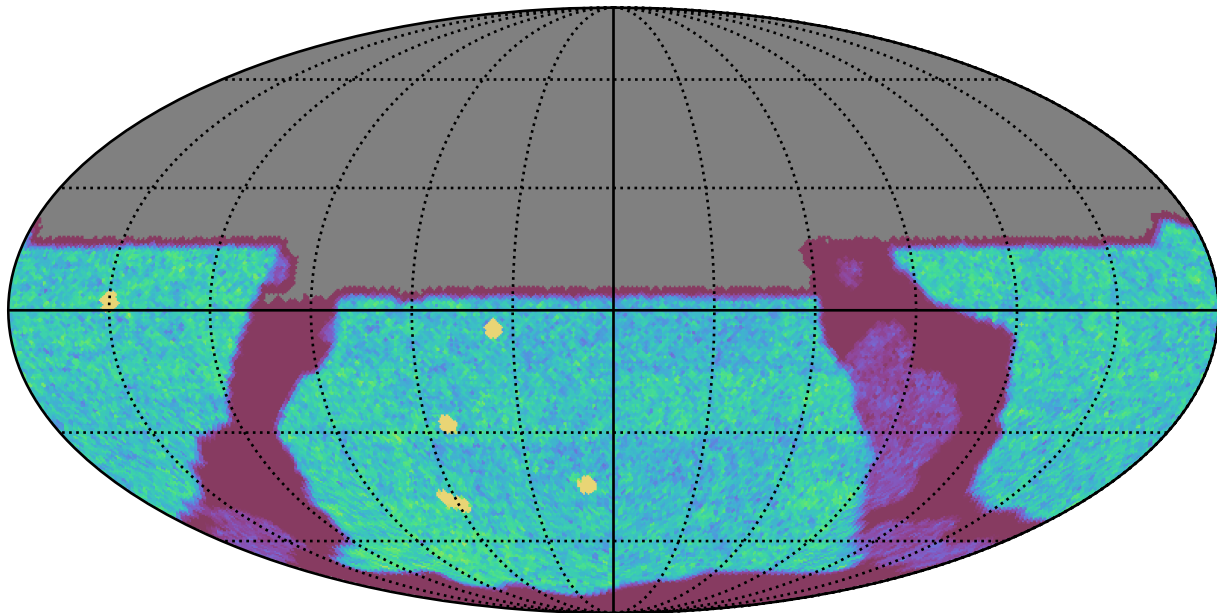
too_ignore_5_1v3.4_10yrs All sky u band: NVisits
