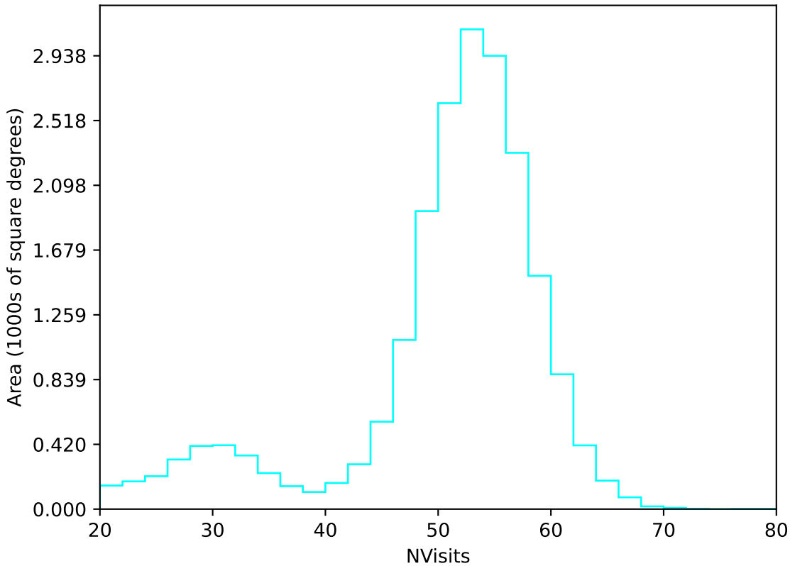
too_ignore_5_1v3.4_10yrs All sky u band: NVisits
