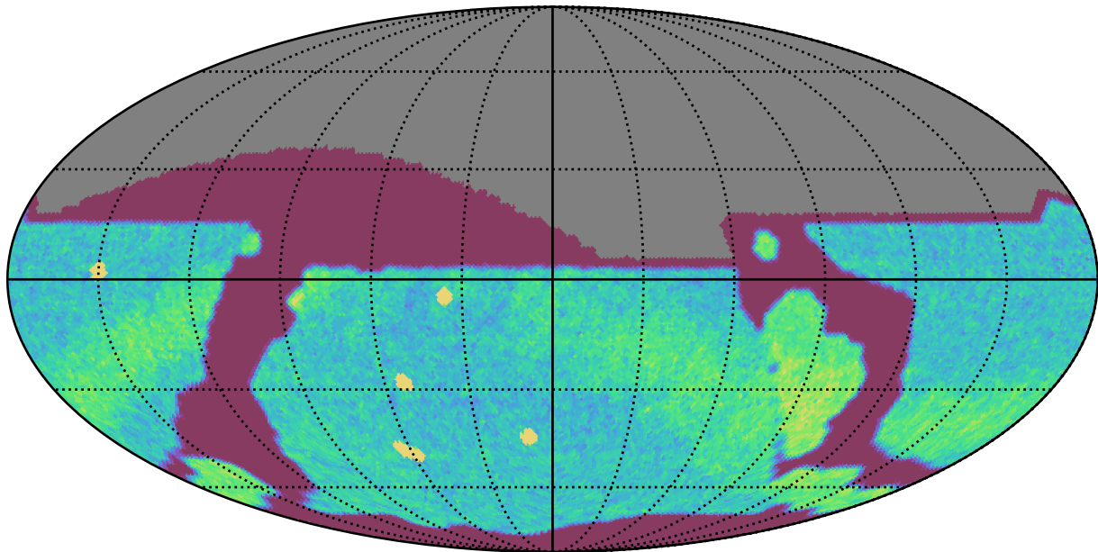
too_ignore_5_1v3.4_10yrs All sky r band: NVisits
