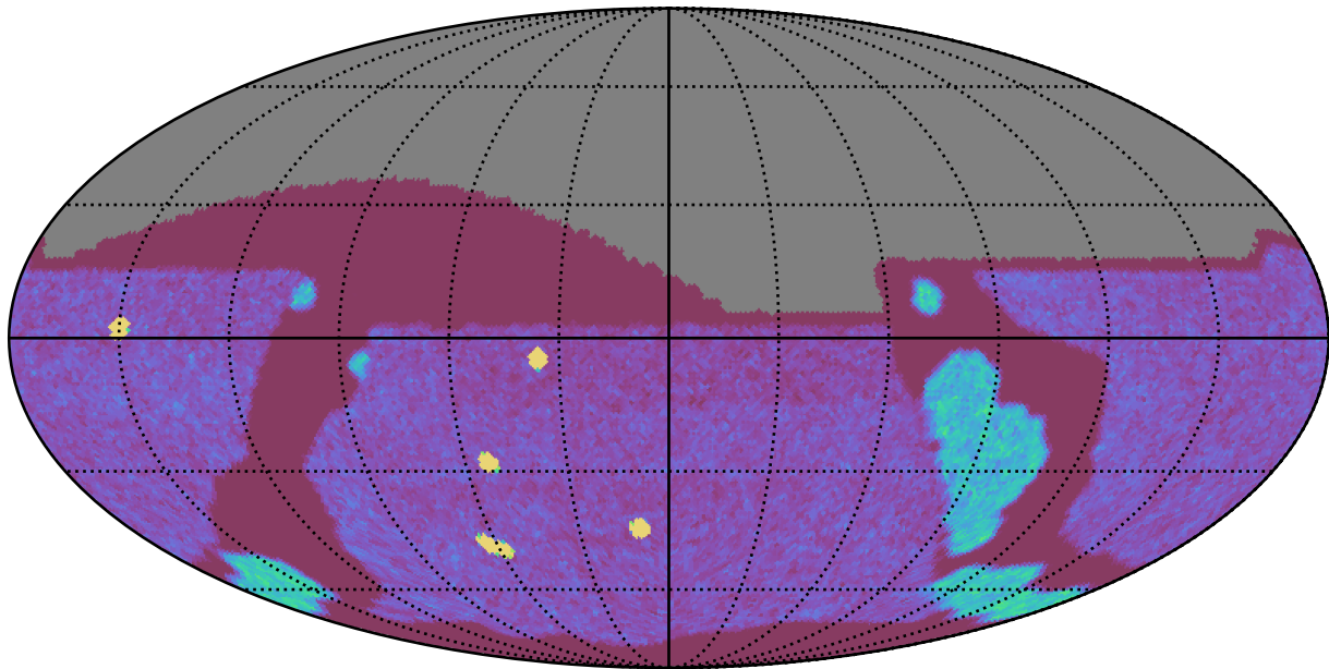
too_ignore_5_1v3.4_10yrs All sky g band: NVisits
