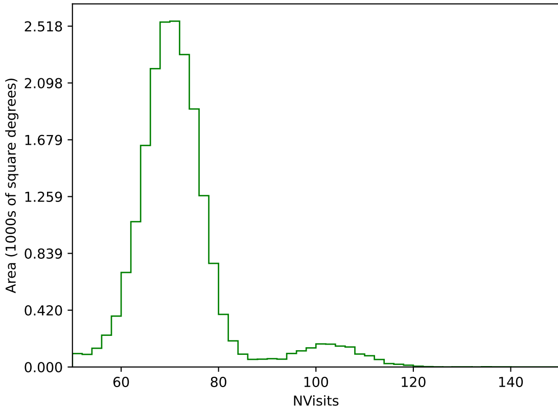
too_ignore_5_1v3.4_10yrs All sky g band: NVisits
