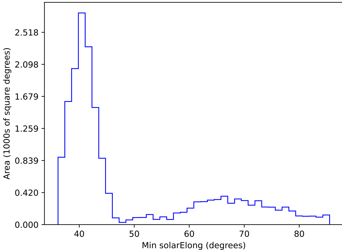
too_ignore_5_1v3.4_10yrs WFD z band: Min solarElong
