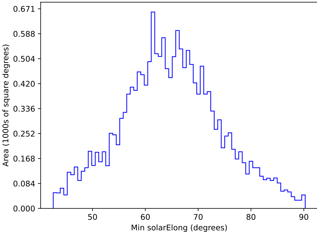
too_ignore_5_1v3.4_10yrs WFD y band: Min solarElong
