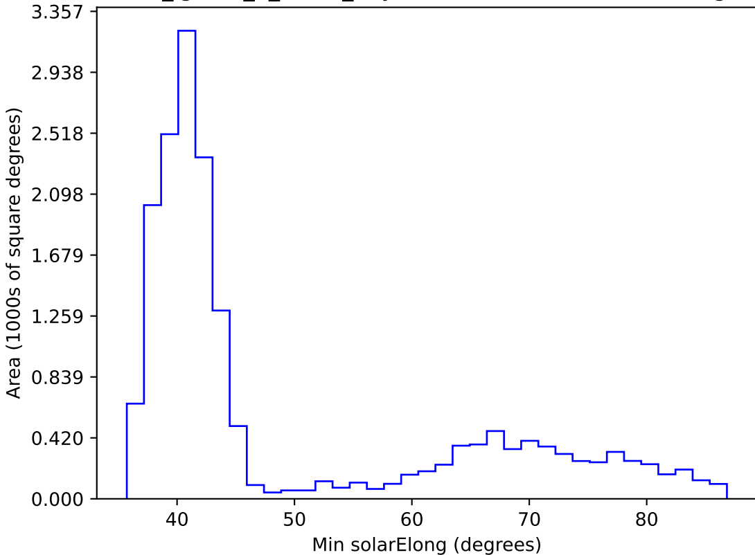
too_ignore_5_1v3.4_10yrs WFD i band: Min solarElong
