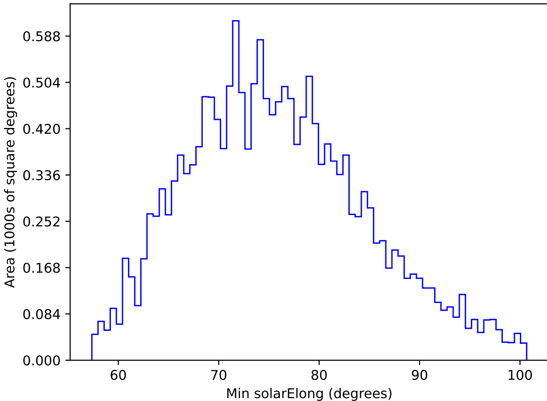
too_ignore_5_1v3.4_10yrs WFD g band: Min solarElong
