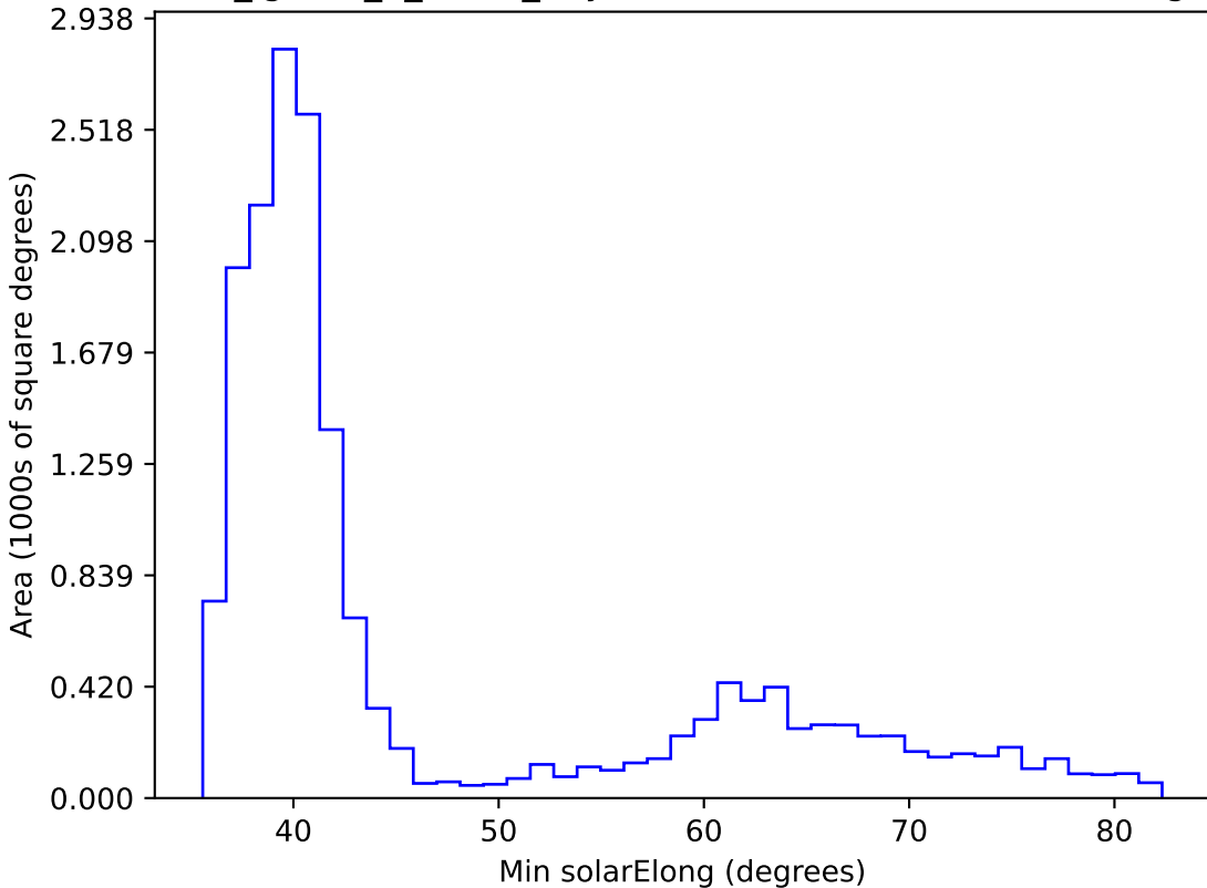
too_ignore_5_1v3.4_10yrs WFD all bands: Min solarElong
