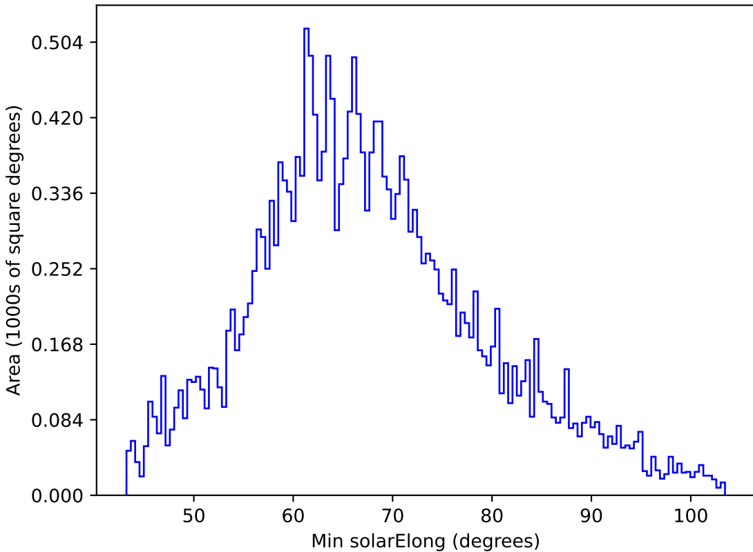
too_ignore_5_1v3.4_10yrs All sky y band: Min solarElong
