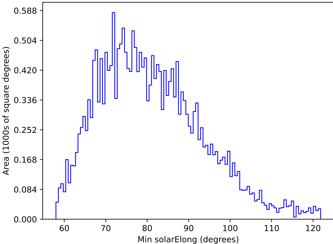
too_ignore_5_1v3.4_10yrs All sky u band: Min solarElong
