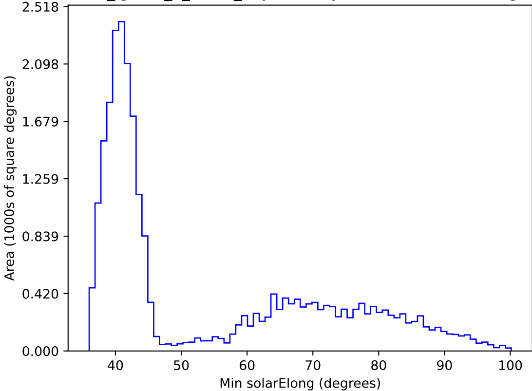
too_ignore_5_1v3.4_10yrs All sky i band: Min solarElong
