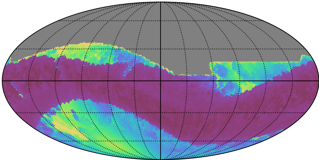
too_ignore_5_1v3.4_10yrs All sky all bands: Min solarElong
