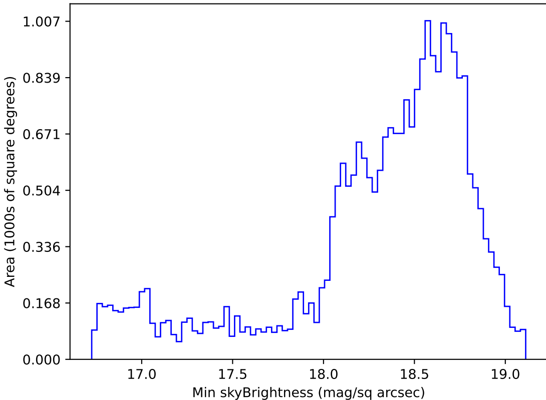
too_ignore_5_1v3.4_10yrs Yr 1 z band: Min skyBrightness
