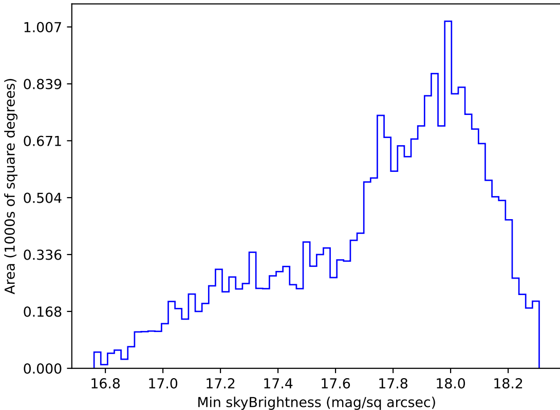
too_ignore_5_1v3.4_10yrs Yr 1 y band: Min skyBrightness
